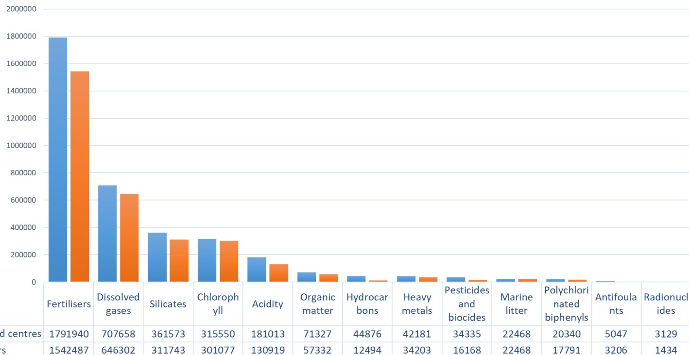
CDIS per EMODnet Chemistry chemical groups (P36)
